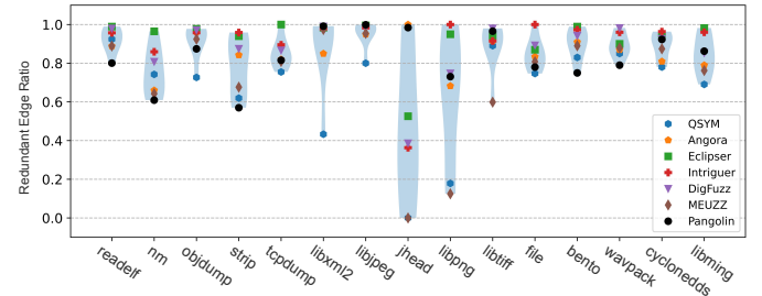
Fig. 3. Redundant edge ratio of studied fuzzers
