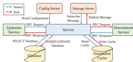
Fig. 6: Source and Sink Types of Microservice Services
