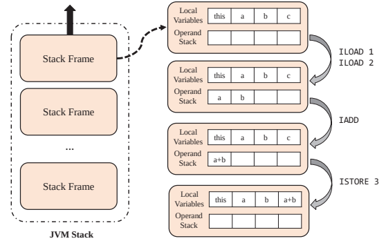
Fig. 1: JVM Execution Model
