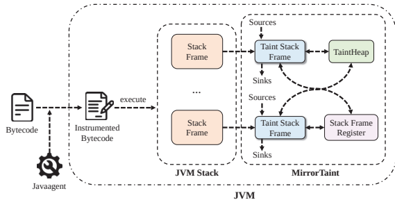
Fig. 4: The Overall Workflow of MirrorTaint
