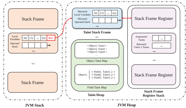
Fig. 5: Data Structures for MirrorTaint
